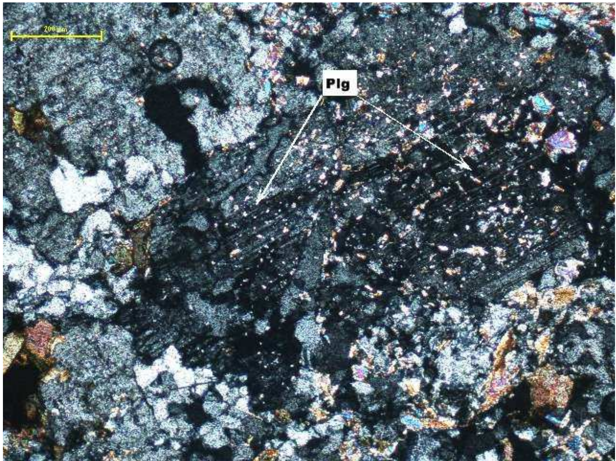
Altered (Sericitized) albitic plagioclase in Soda Granite, Singhum
