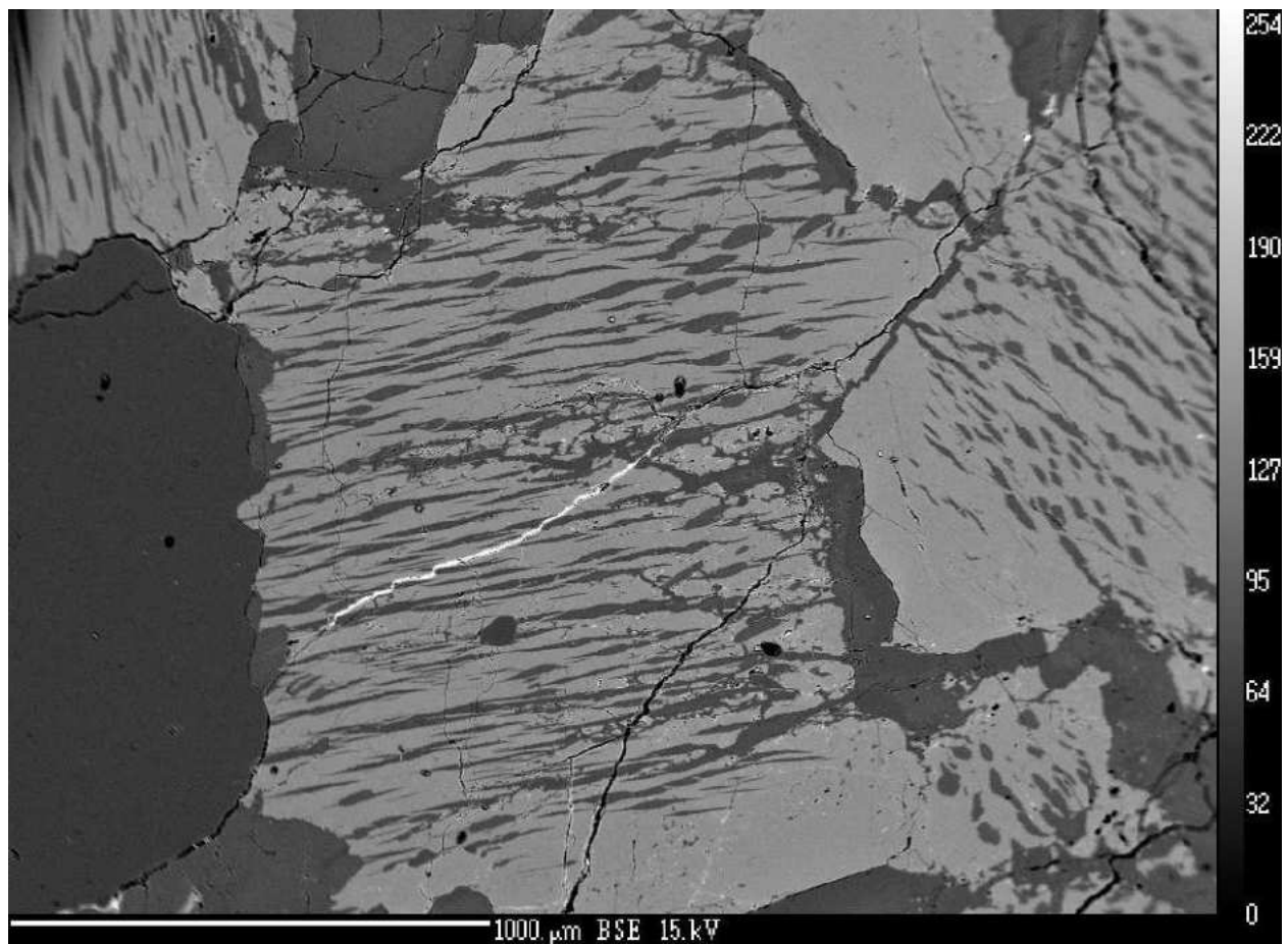
BSE- image of Perthite, Sholayar Syenite Complex, Kerala
